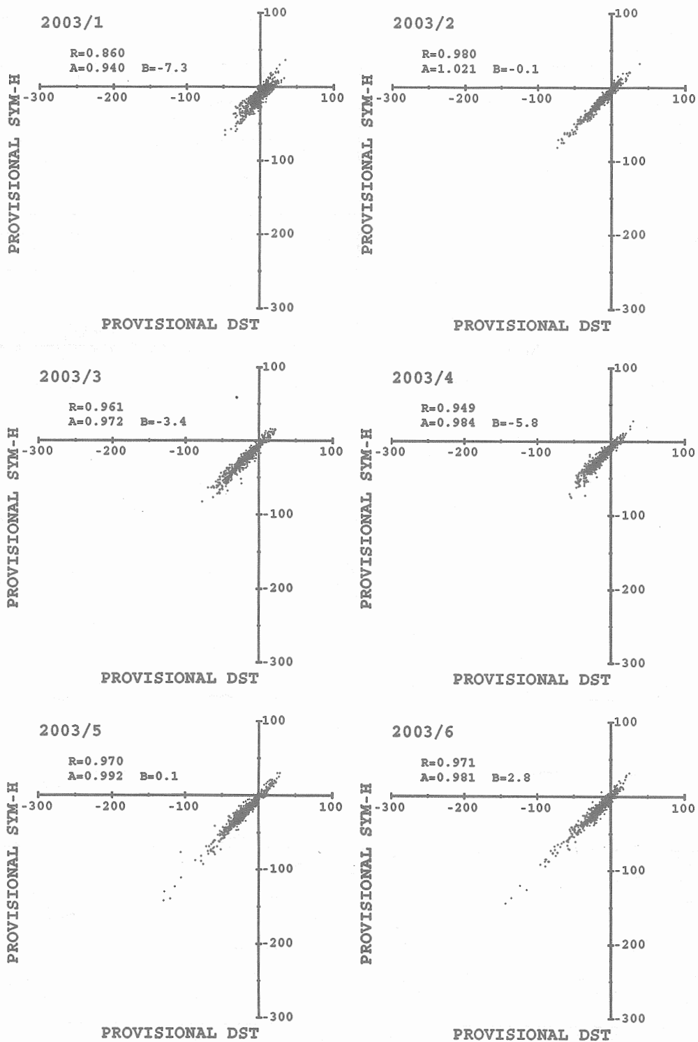
Figure 3a. Correlation plots between the hourly averaged SYM-H and the provisional Dst for January-June, 2003. The correlation coefficients R, the parameters of the regression line A and B (i.e. \text{SYM-H} = A \cdot \text{Dst} + B ) are shown on each panel.
